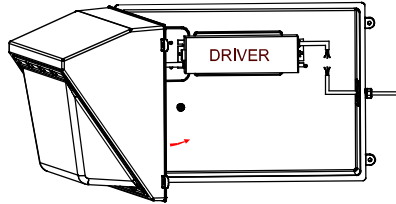
5.Put the cover on the base,join the DC end waterproof connector with each other, and tighten the cover Cover,and screw to fix(pic 5)
